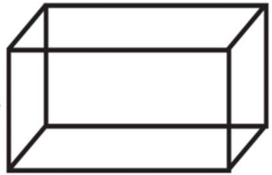
Rectangular Prism
