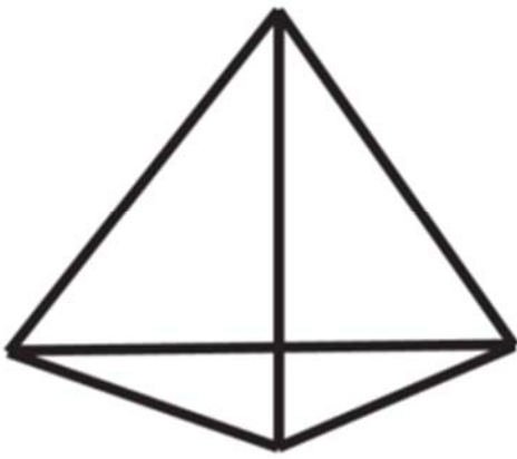
Tetrahedron (Triangular Pyramid)
