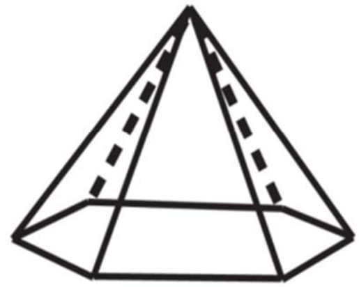
Hexagonal Pyramid
