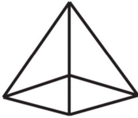
Square Pyramid
