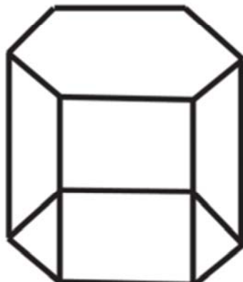
Hexagonal Prism
