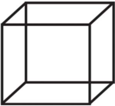
Cube
