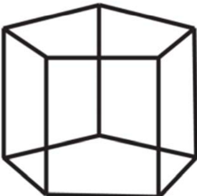
Pentagonal Prism
