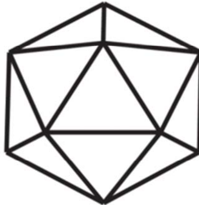
Icosahedron
