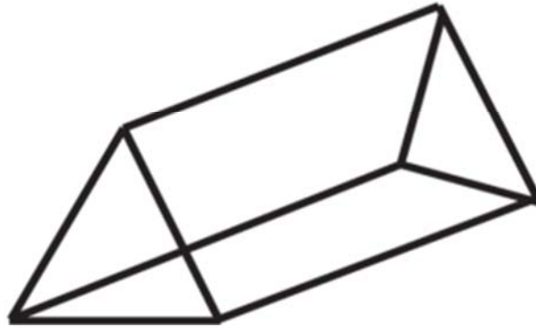
Triangular Prism
